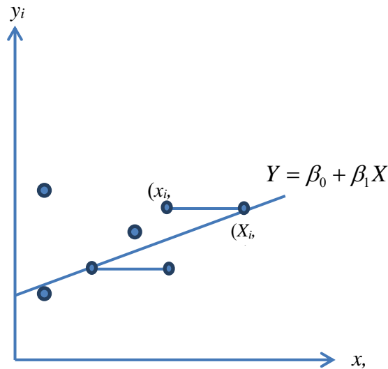
Reverse regression
