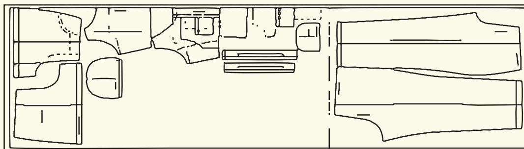
DUNGAREE PATTERN LAYOUT ON FOLD
