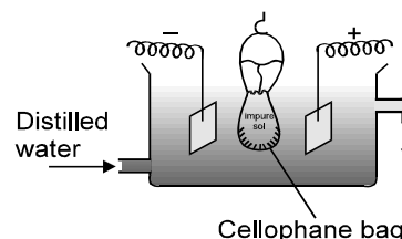
Fig. : An apparatus for electro-dialysis.
