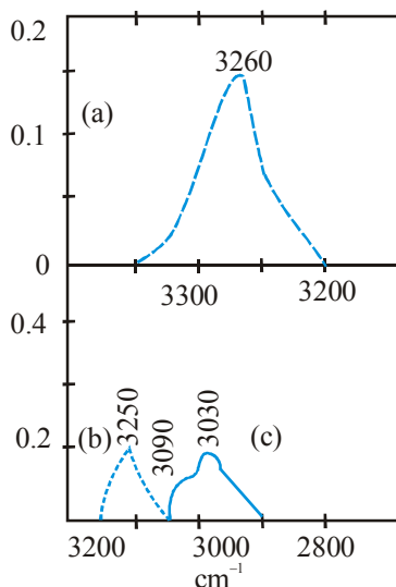
(Infrared spectra of (a) acetylene in liquid solution, (b) acetylene on porous silica glass (c) acetylene on porous silica glass coated with palladium)
